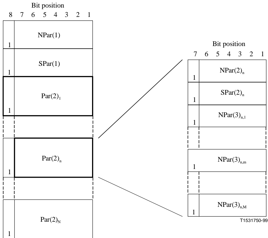
FIGURE 8/G.994.1
