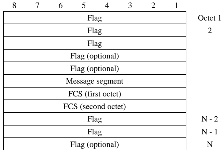
FIGURE 5/G.994.1 Frame structure
